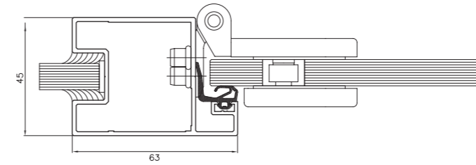
Door stud and upper crossbar – view
