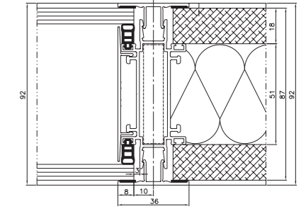
92 mm wall - vertical view
