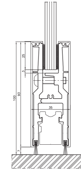
Mobile and door leaf – lower cross section
