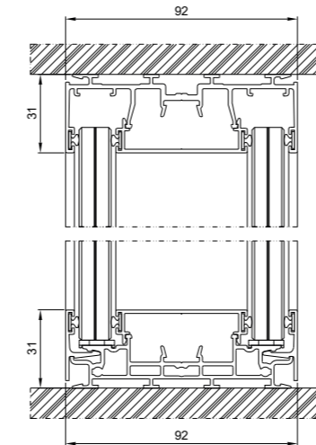
Internal partition, vertical cross-section
