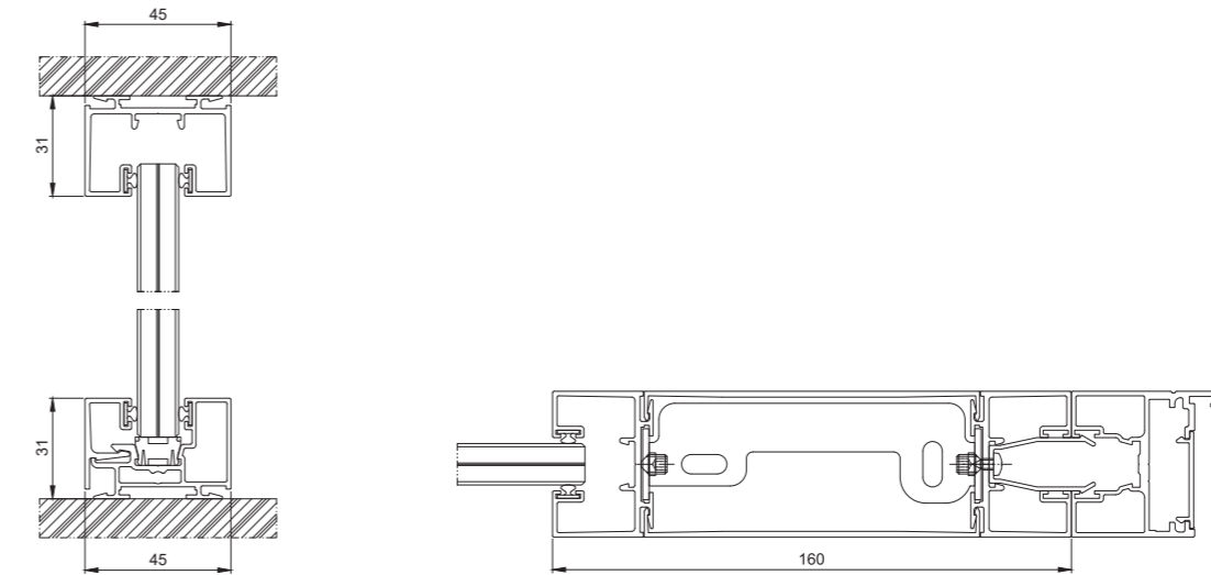
Internal partition, vertical cross-section
