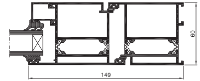
door – cross-section MB-60
