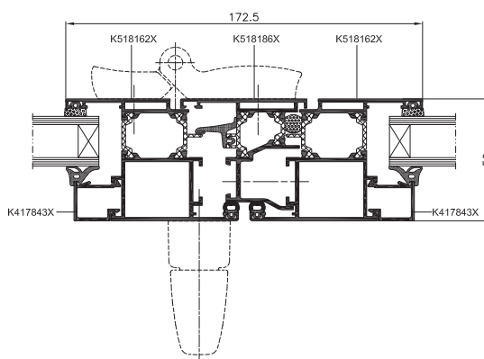
folding door – cross-section
